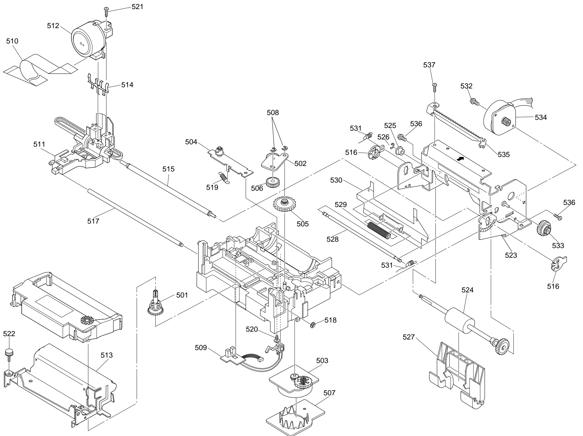
EXPLODED DIAGRAM FOR TM-U200B NO.2
